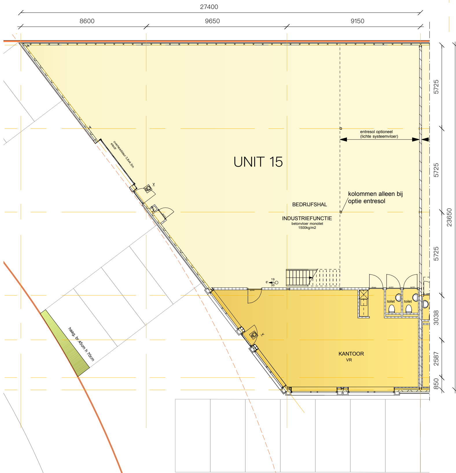
UNIT 15 begane grond
