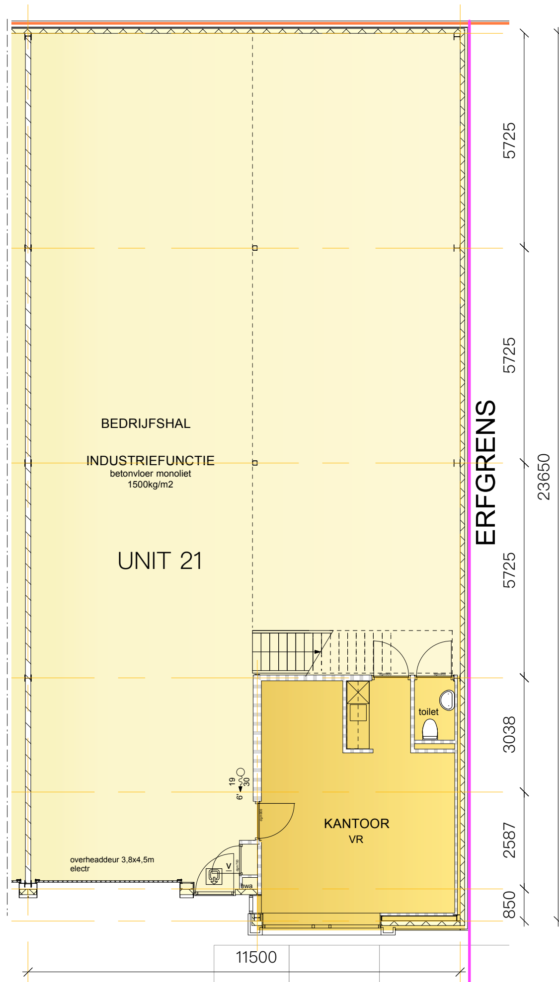
UNIT 21 begane grond
