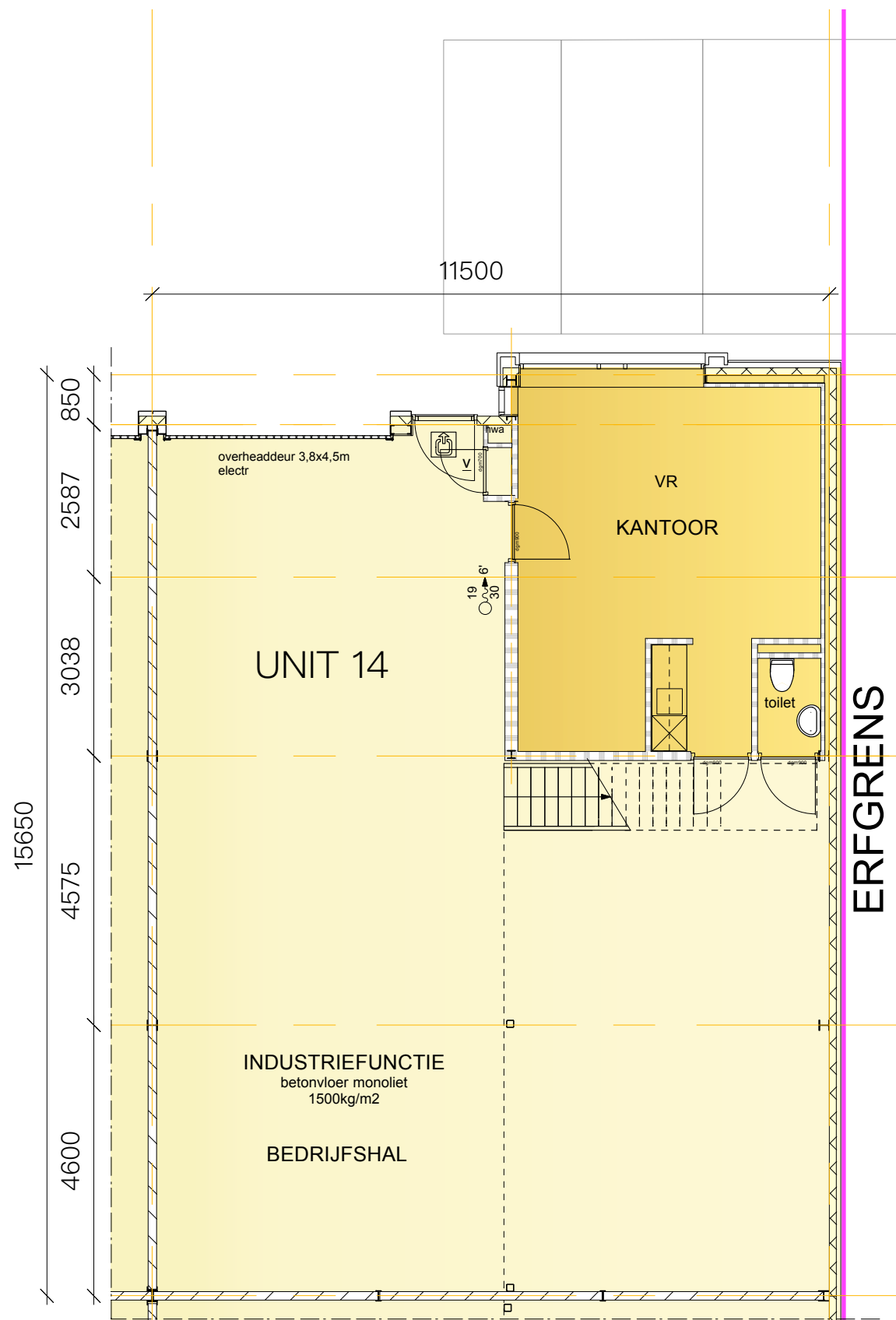
UNIT 14 begane grond
