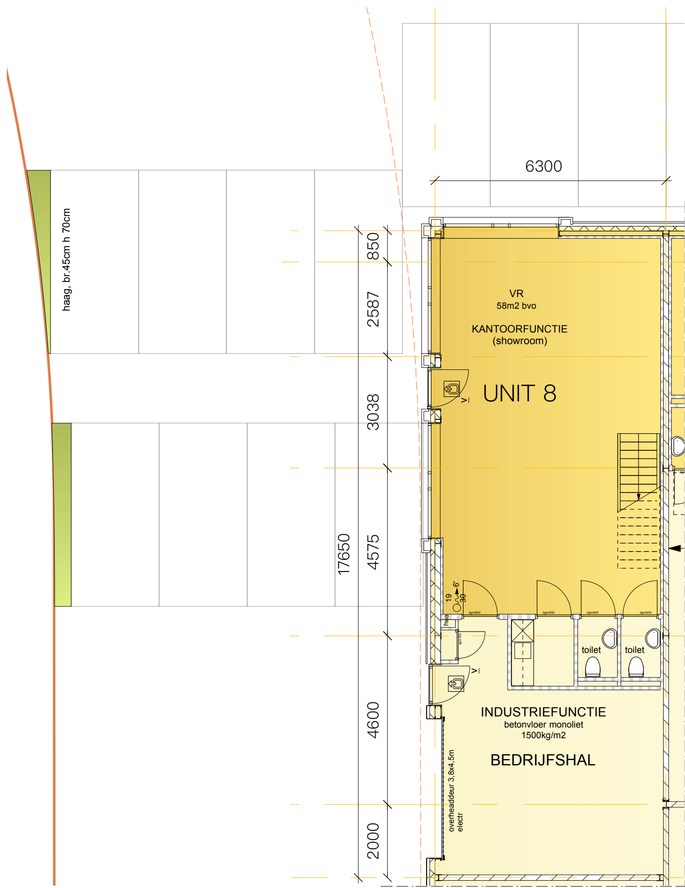
UNIT 8 begane grond
